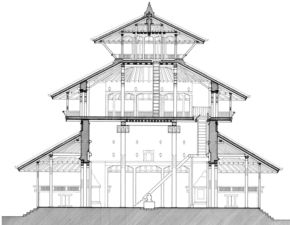
KASTHAMANDAP ELEVATION | WOLFGANG KORN
